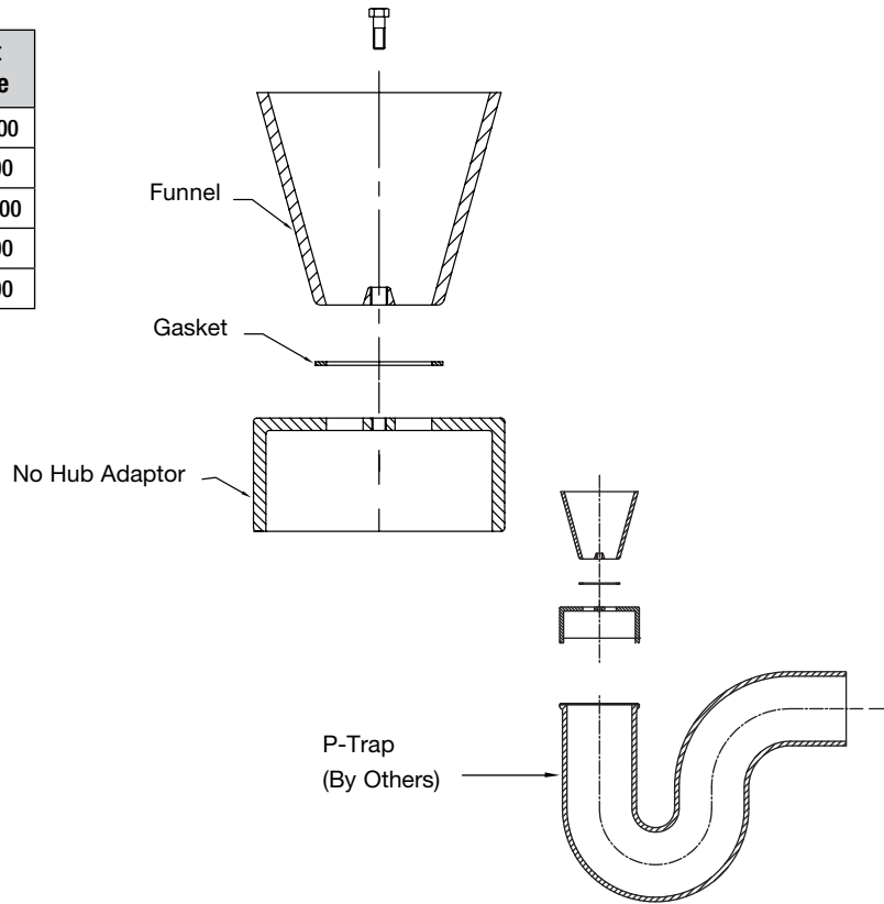
Typical Installation
